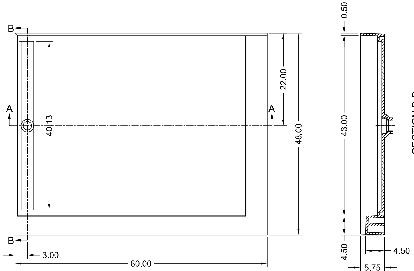
SECTION B-B
